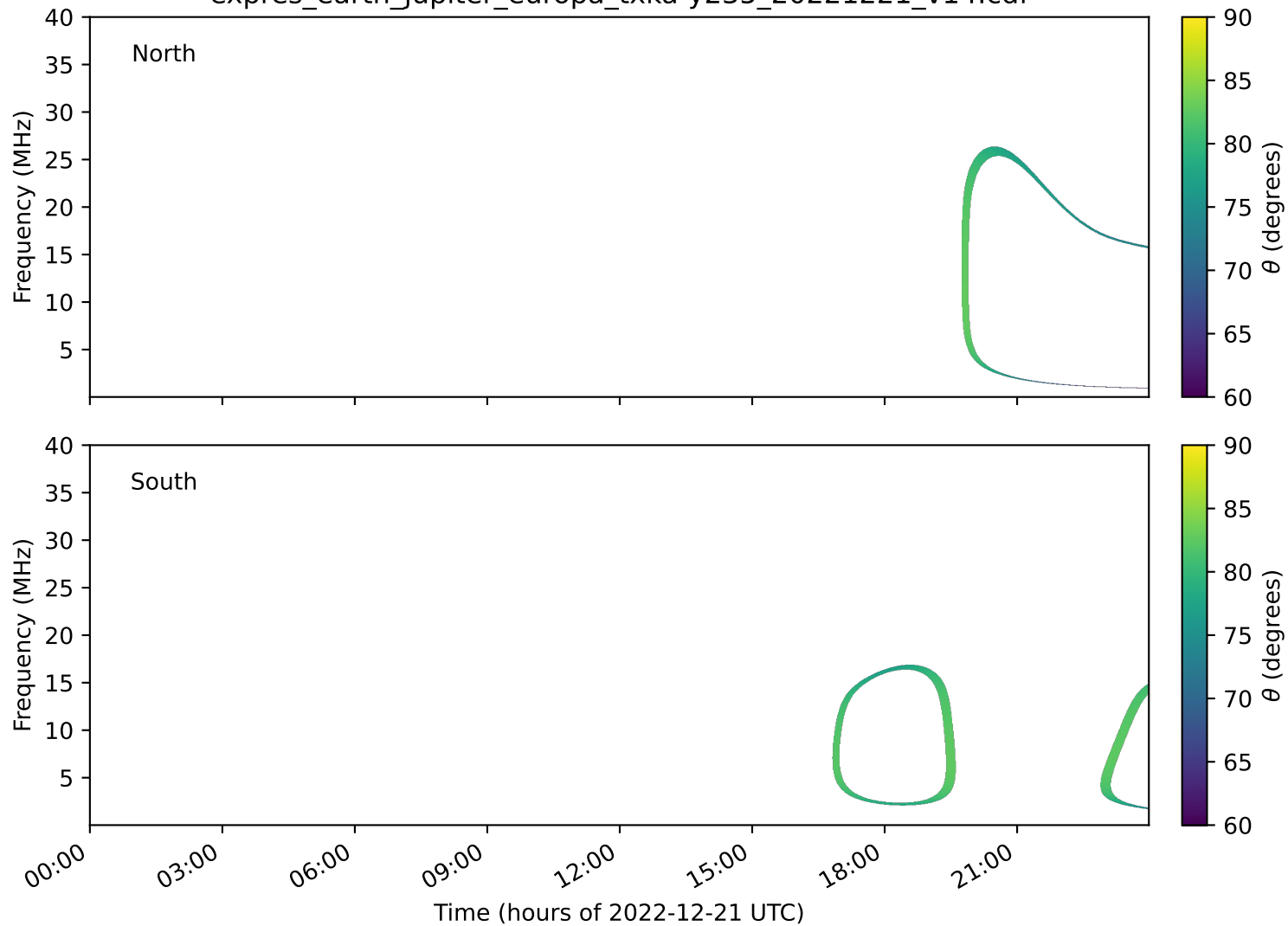
expres_earth_jupiter_europa_txka-y235_20221221_v14.cdf
