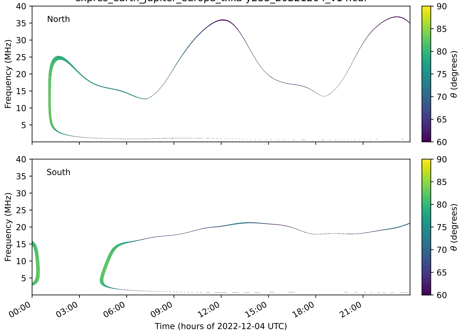
expres_earth_jupiter_europa_txka-y235_20221204_v14.cdf
