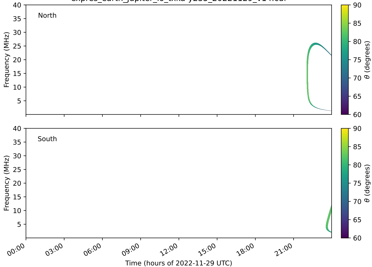
expres_earth_jupiter_io_txka-y235_20221129_v14.cdf
