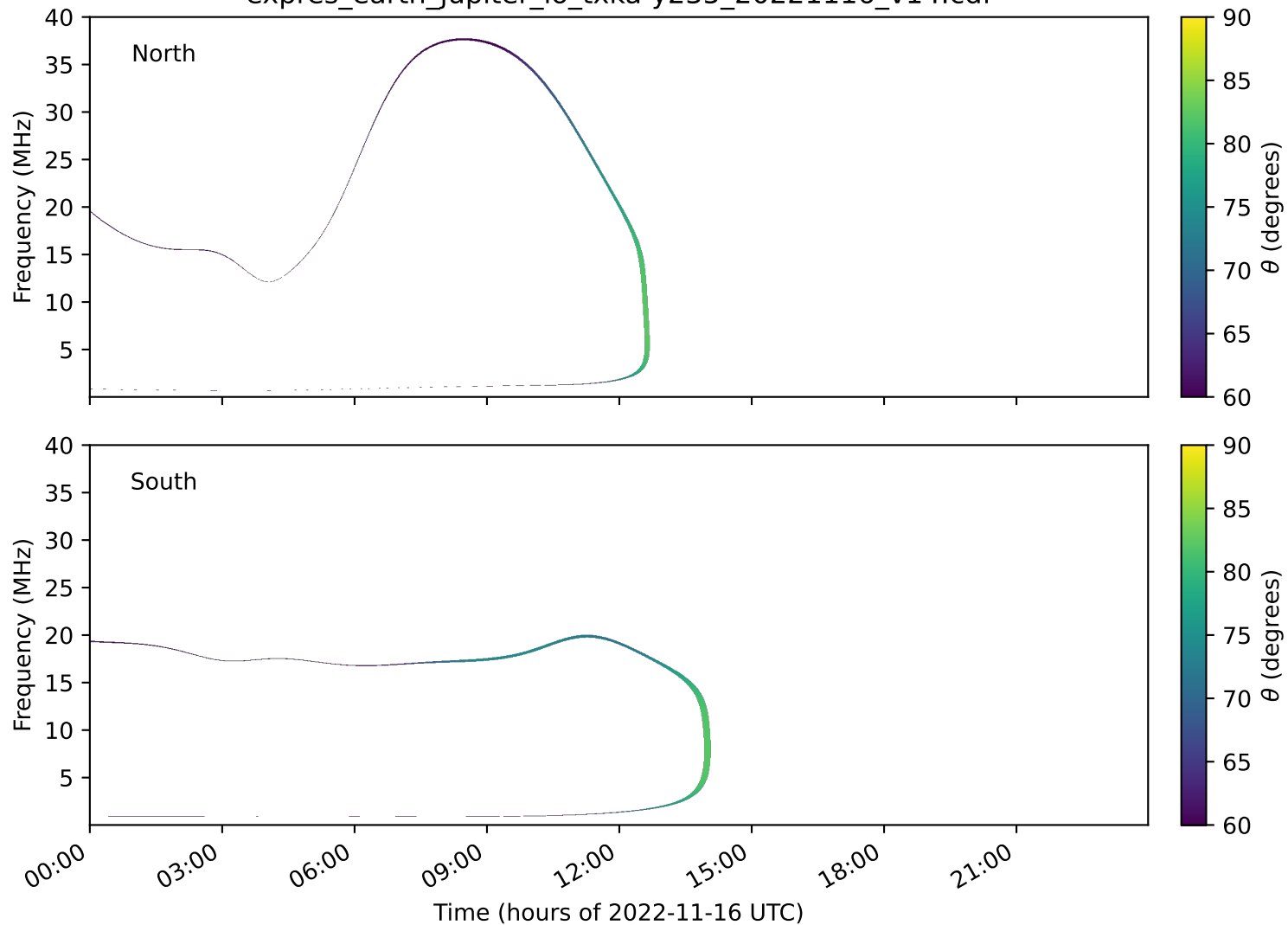
expres_earth_jupiter_io_txka-y235_20221116_v14.cdf
