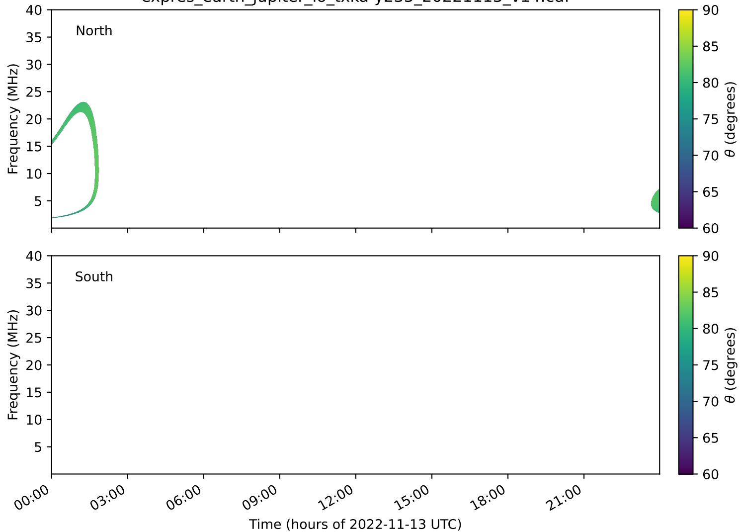
expres_earth_jupiter_io_txka-y235_20221113_v14.cdf
