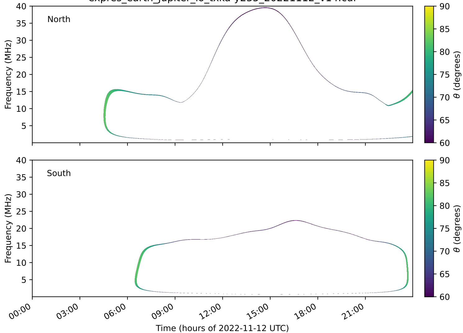
expres_earth_jupiter_io_txka-y235_20221112_v14.cdf
