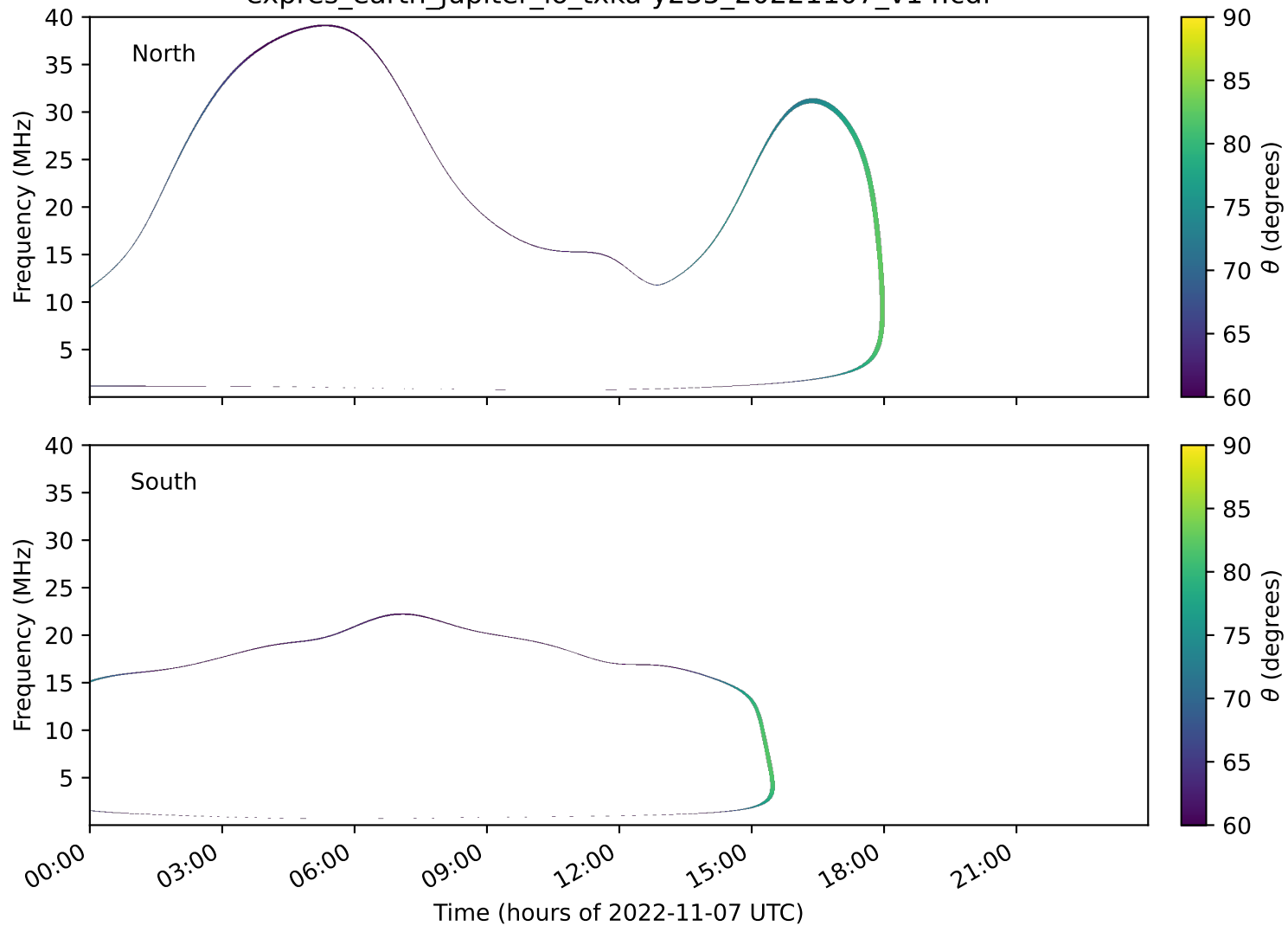
expres_earth_jupiter_io_txka-y235_20221107_v14.cdf
