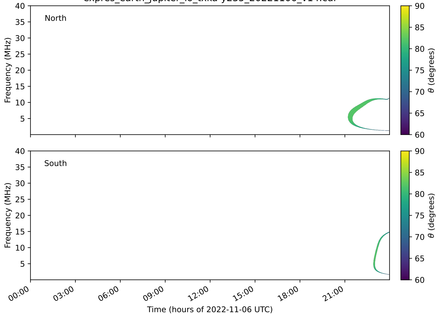
expres_earth_jupiter_io_txka-y235_20221106_v14.cdf
