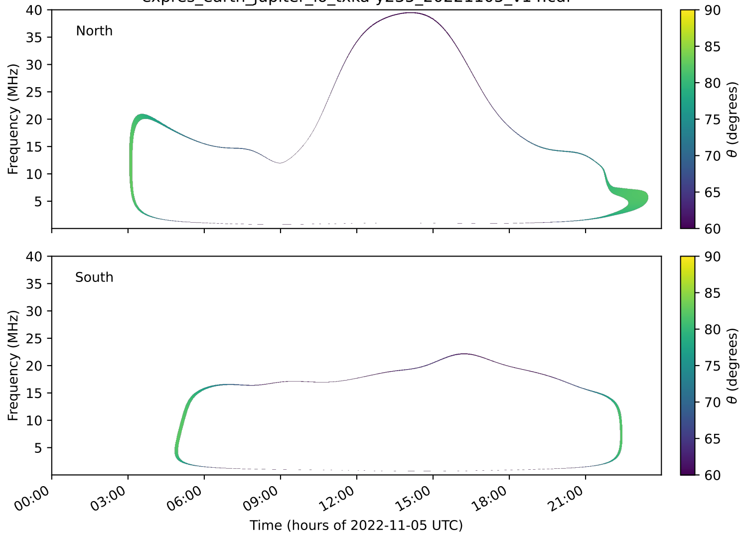
expres_earth_jupiter_io_txka-y235_20221105_v14.cdf
