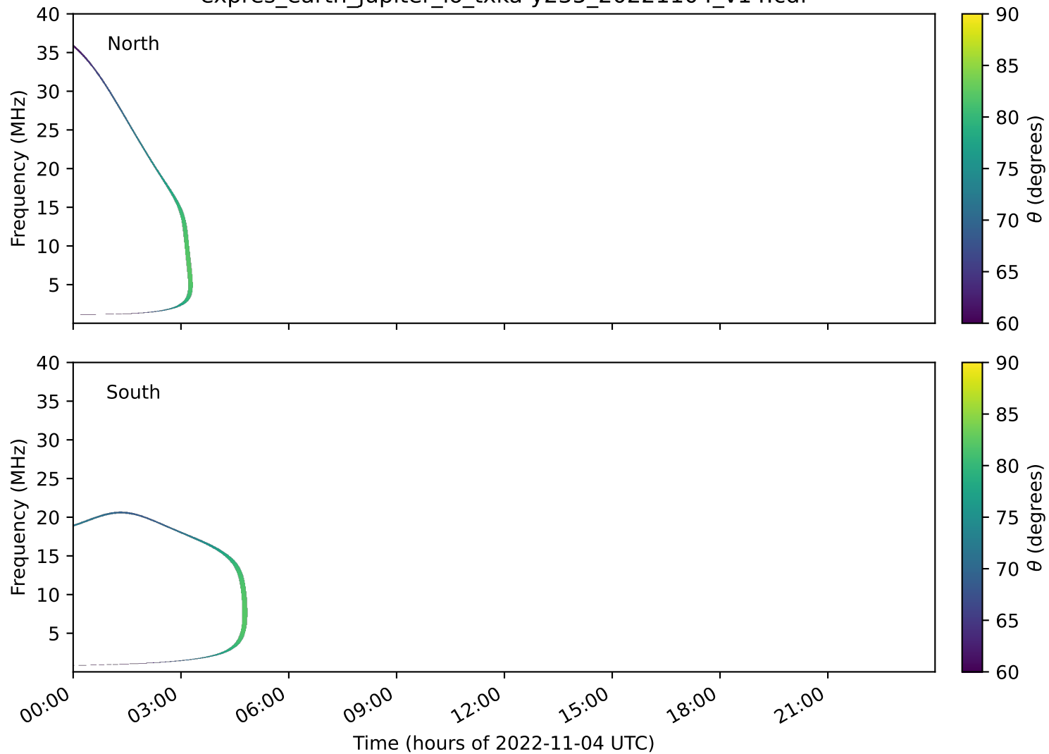
expres_earth_jupiter_io_txka-y235_20221104_v14.cdf
