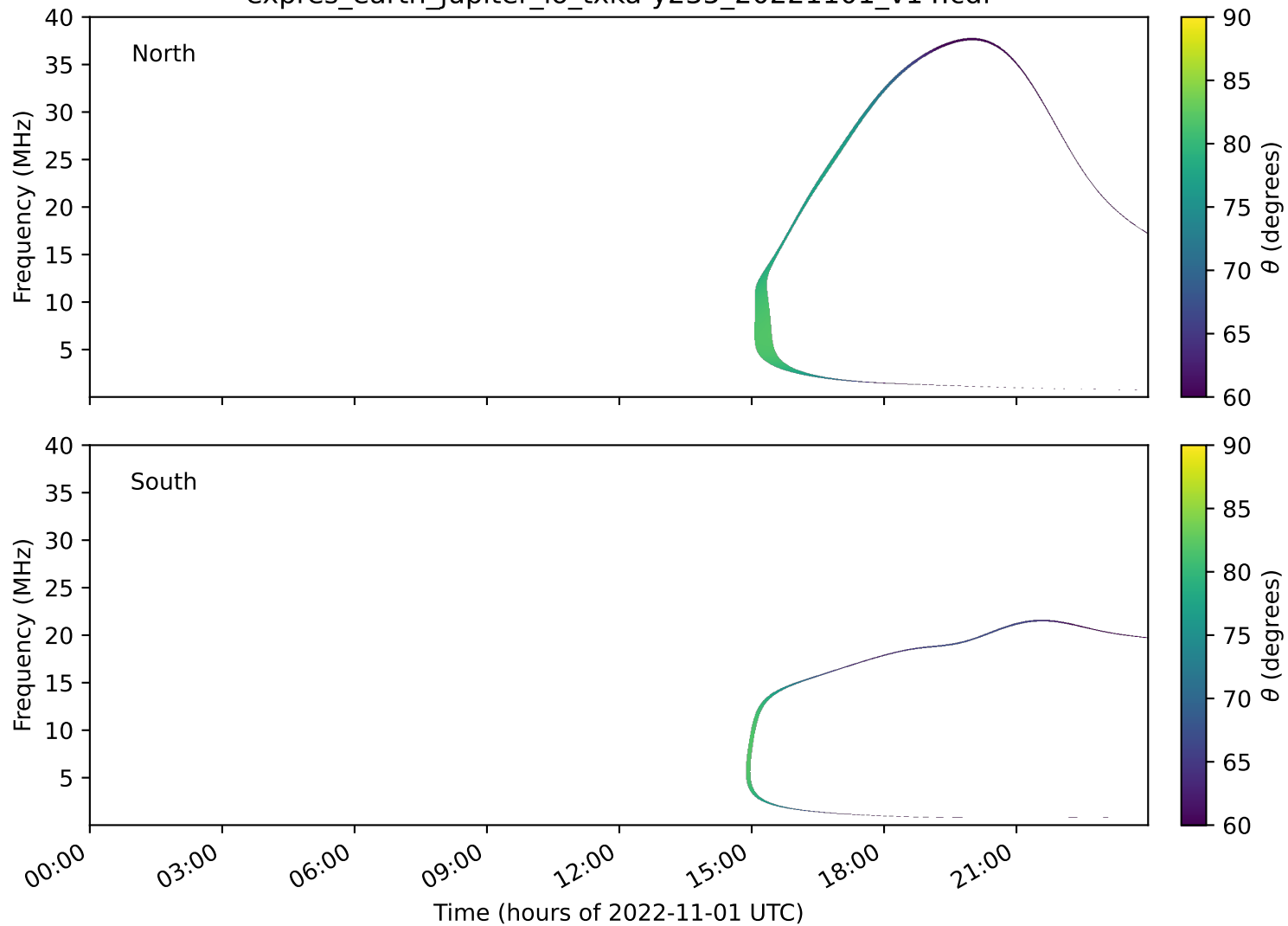
expres_earth_jupiter_io_txka-y235_20221101_v14.cdf
