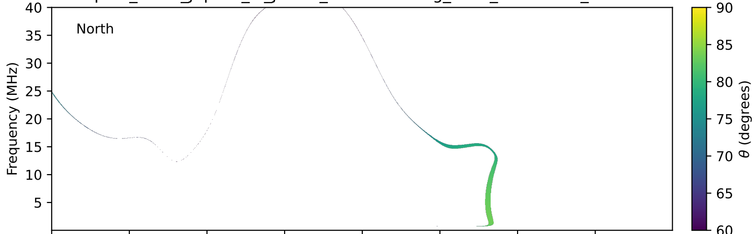
expres_earth_jupiter_io_jrm33_lossc-wid1deg_3kev_20221130_v11.cdf
