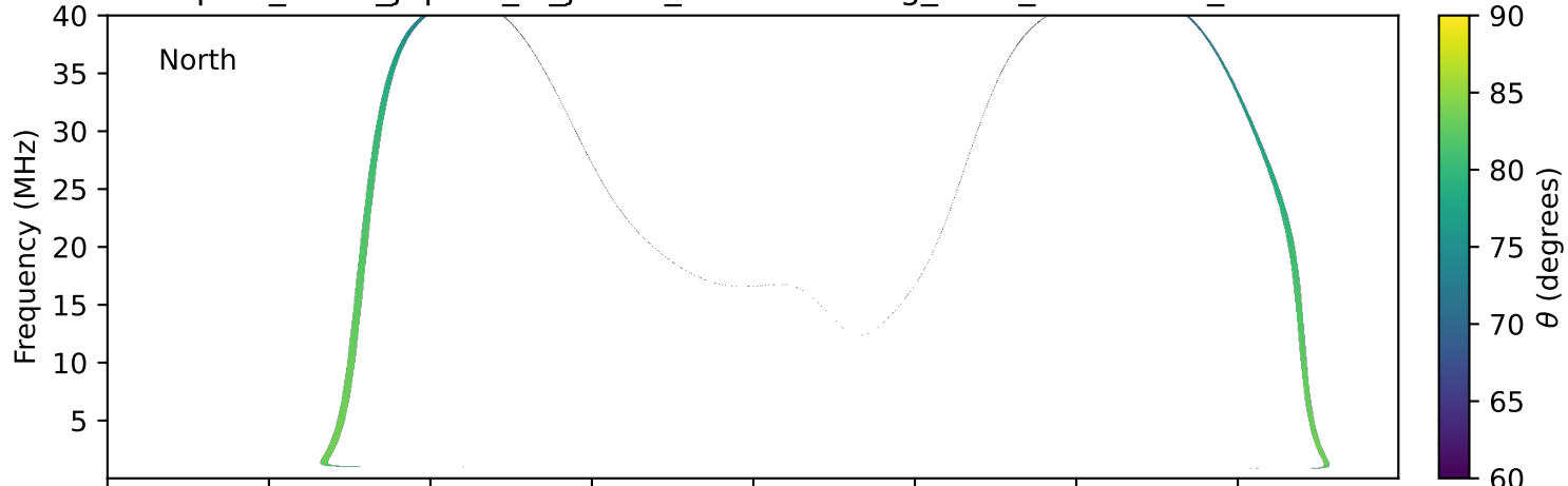
expres_earth_jupiter_io_jrm33_lossc-wid1deg_3kev_20221128_v11.cdf
