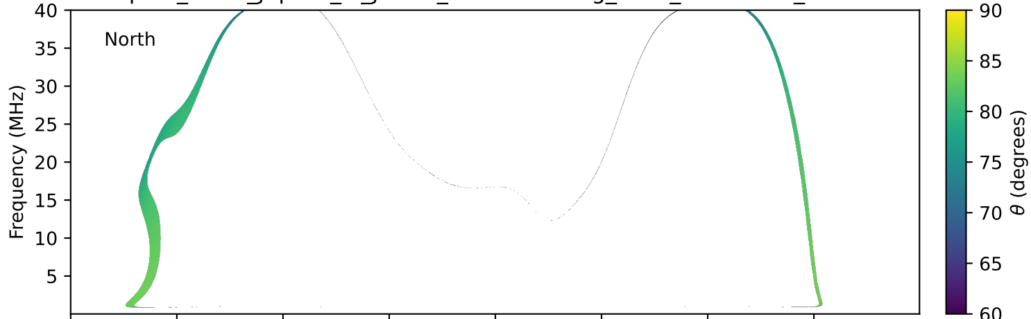
expres_earth_jupiter_io_jrm33_lossc-wid1deg_3kev_20221121_v11.cdf
