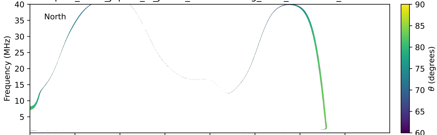
expres_earth_jupiter_io_jrm33_lossc-wid1deg_3kev_20221114_v11.cdf
