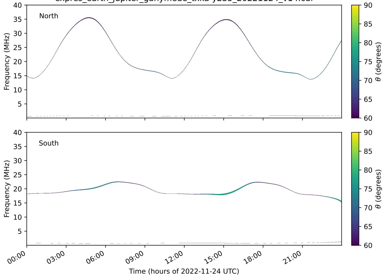
expres_earth_jupiter_ganymede_txka-y235_20221124_v14.cdf
