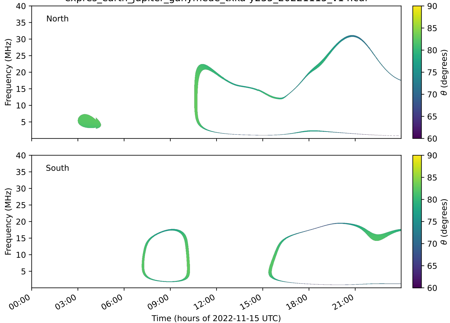
expres_earth_jupiter_ganymede_txka-y235_20221115_v14.cdf
