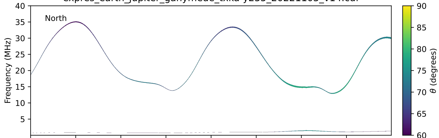
expres_earth_jupiter_ganymede_txka-y235_20221103_v14.cdf
