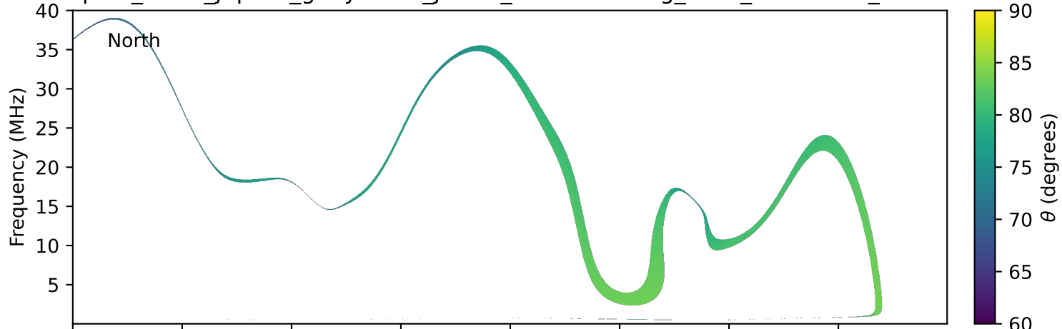
expres_earth_jupiter_ganymede_jrm33_lossc-wid1deg_3kev_20221118_v11.cdf
