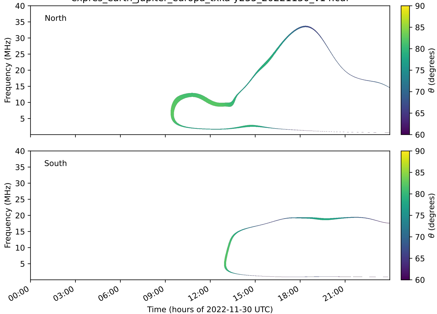
expres_earth_jupiter_europa_txka-y235_20221130_v14.cdf
