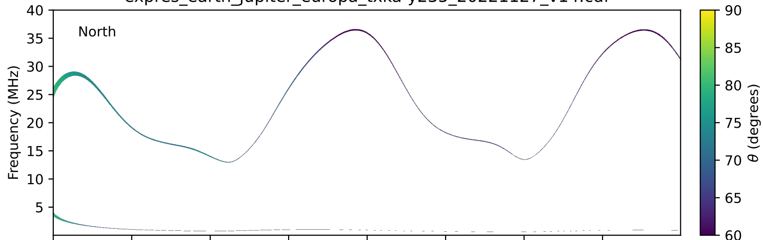
expres_earth_jupiter_europa_txka-y235_20221127_v14.cdf
