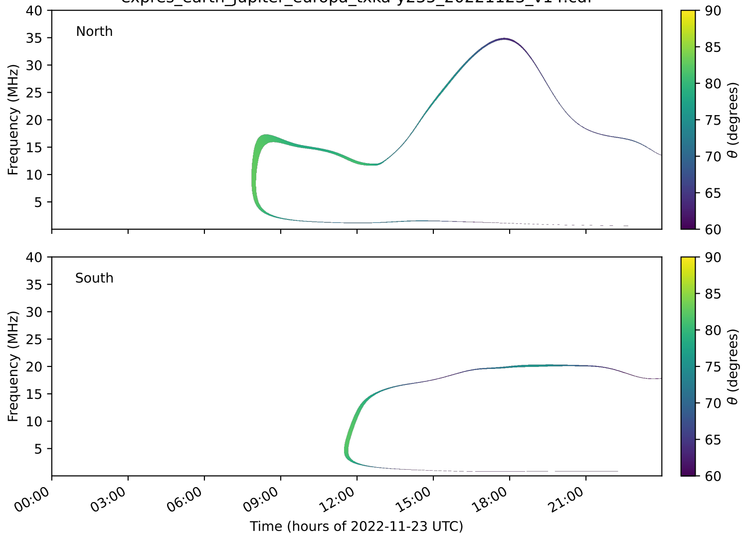
expres_earth_jupiter_europa_txka-y235_20221123_v14.cdf
