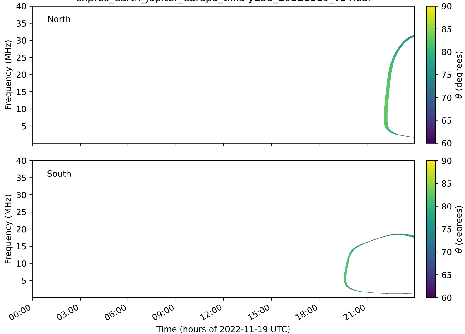
expres_earth_jupiter_europa_txka-y235_20221119_v14.cdf
