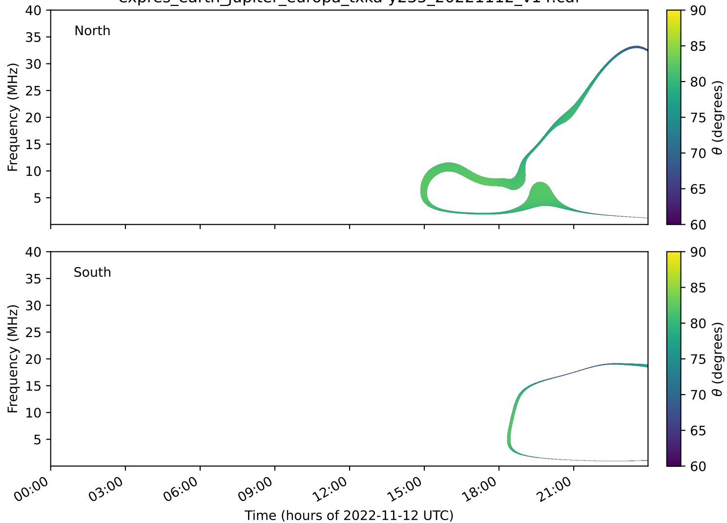
expres_earth_jupiter_europa_txka-y235_20221112_v14.cdf
