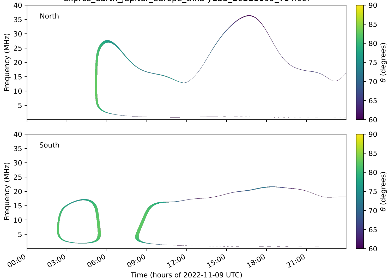
expres_earth_jupiter_europa_txka-y235_20221109_v14.cdf
