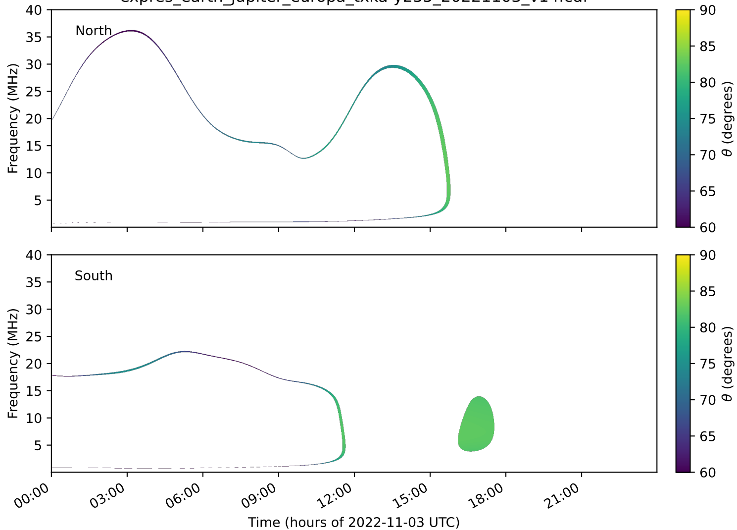
expres_earth_jupiter_europa_txka-y235_20221103_v14.cdf
