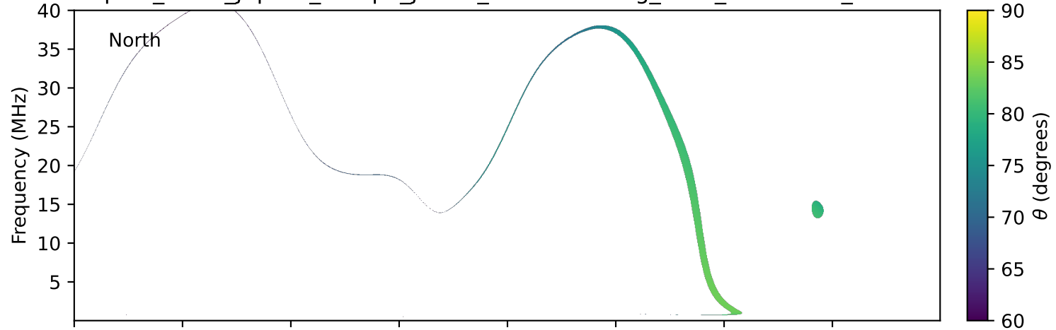
expres_earth_jupiter_europa_jrm33_lossc-wid1deg_3kev_20221110_v11.cdf
