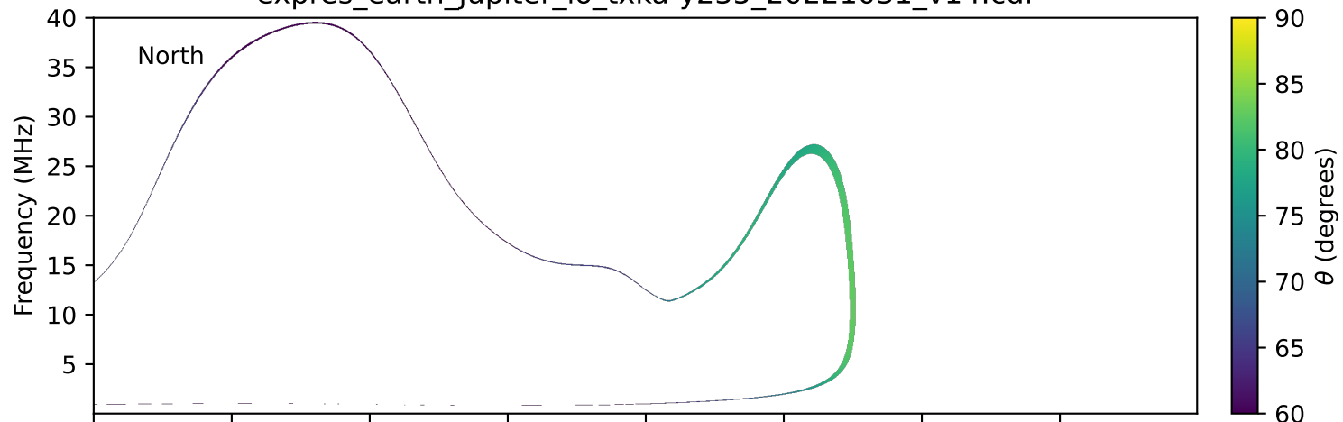
expres_earth_jupiter_io_txka-y235_20221031_v14.cdf
