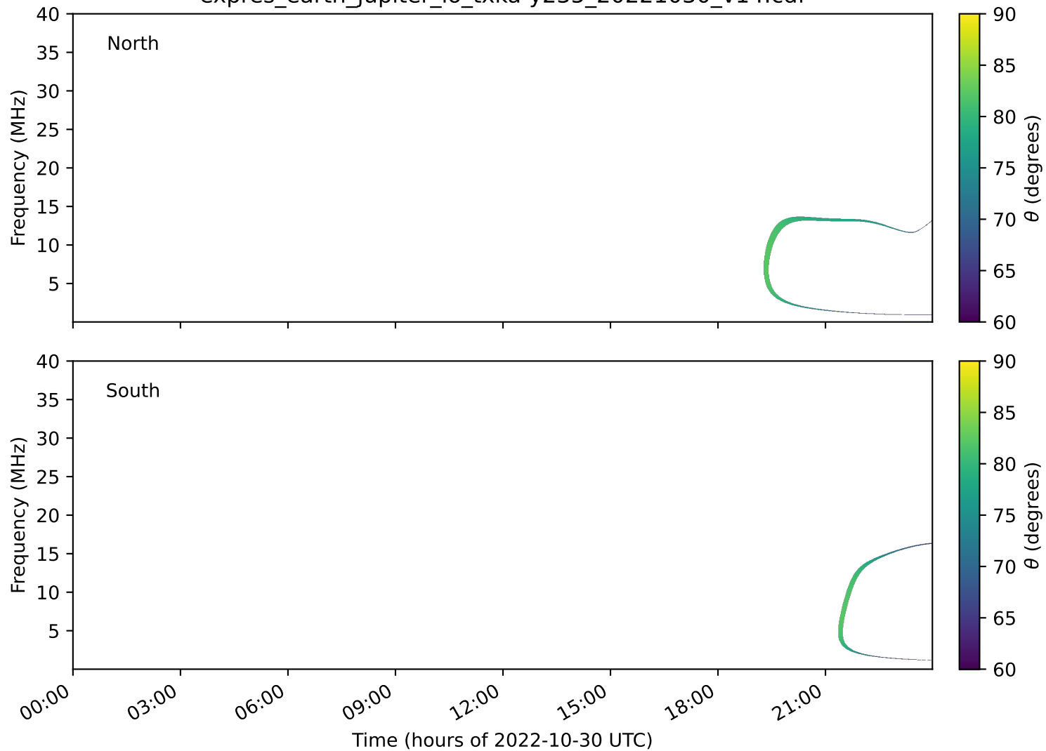
expres_earth_jupiter_io_txka-y235_20221030_v14.cdf
