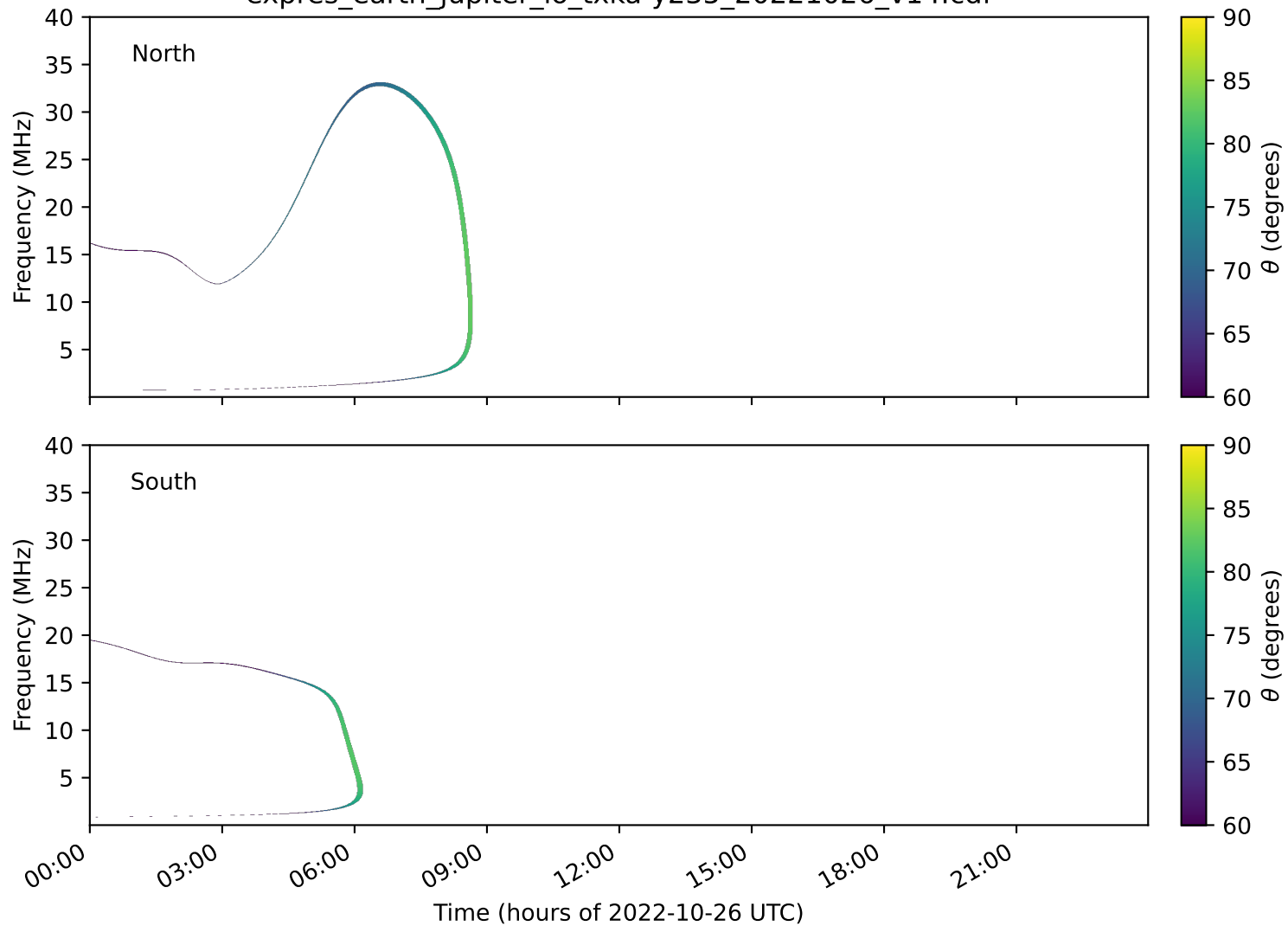
expres_earth_jupiter_io_txka-y235_20221026_v14.cdf
