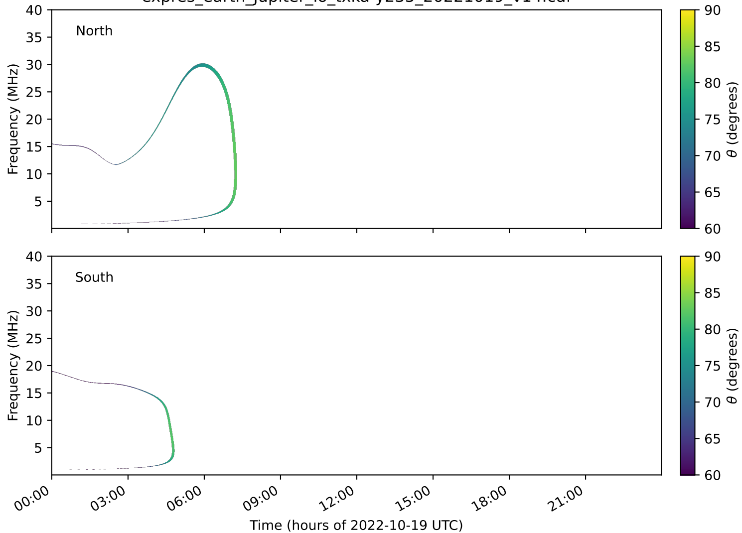
expres_earth_jupiter_io_txka-y235_20221019_v14.cdf
