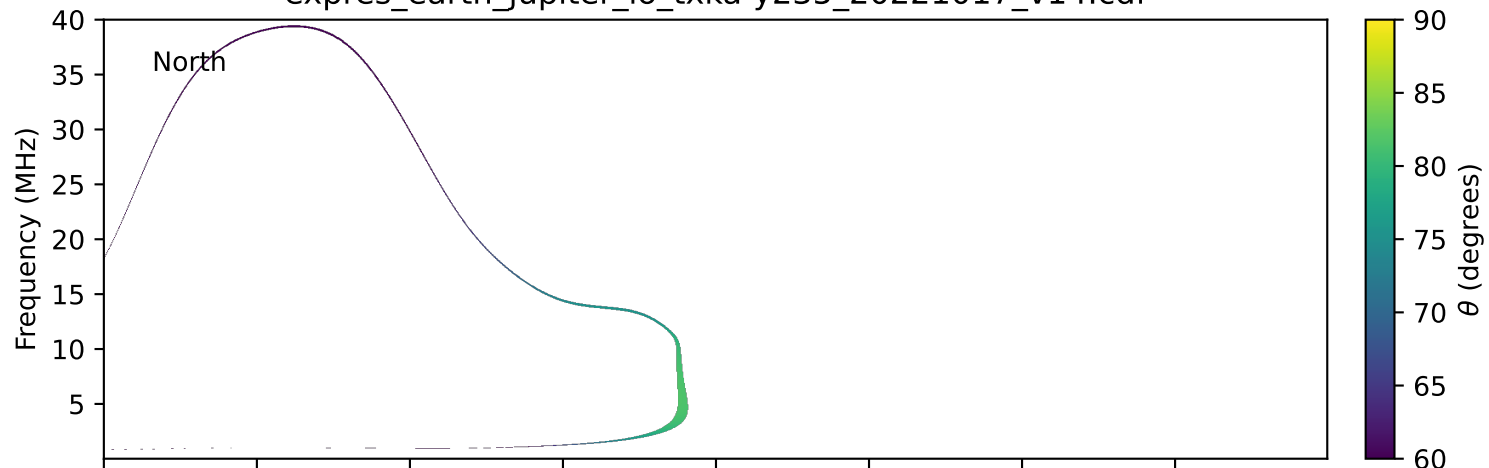
expres_earth_jupiter_io_txka-y235_20221017_v14.cdf
