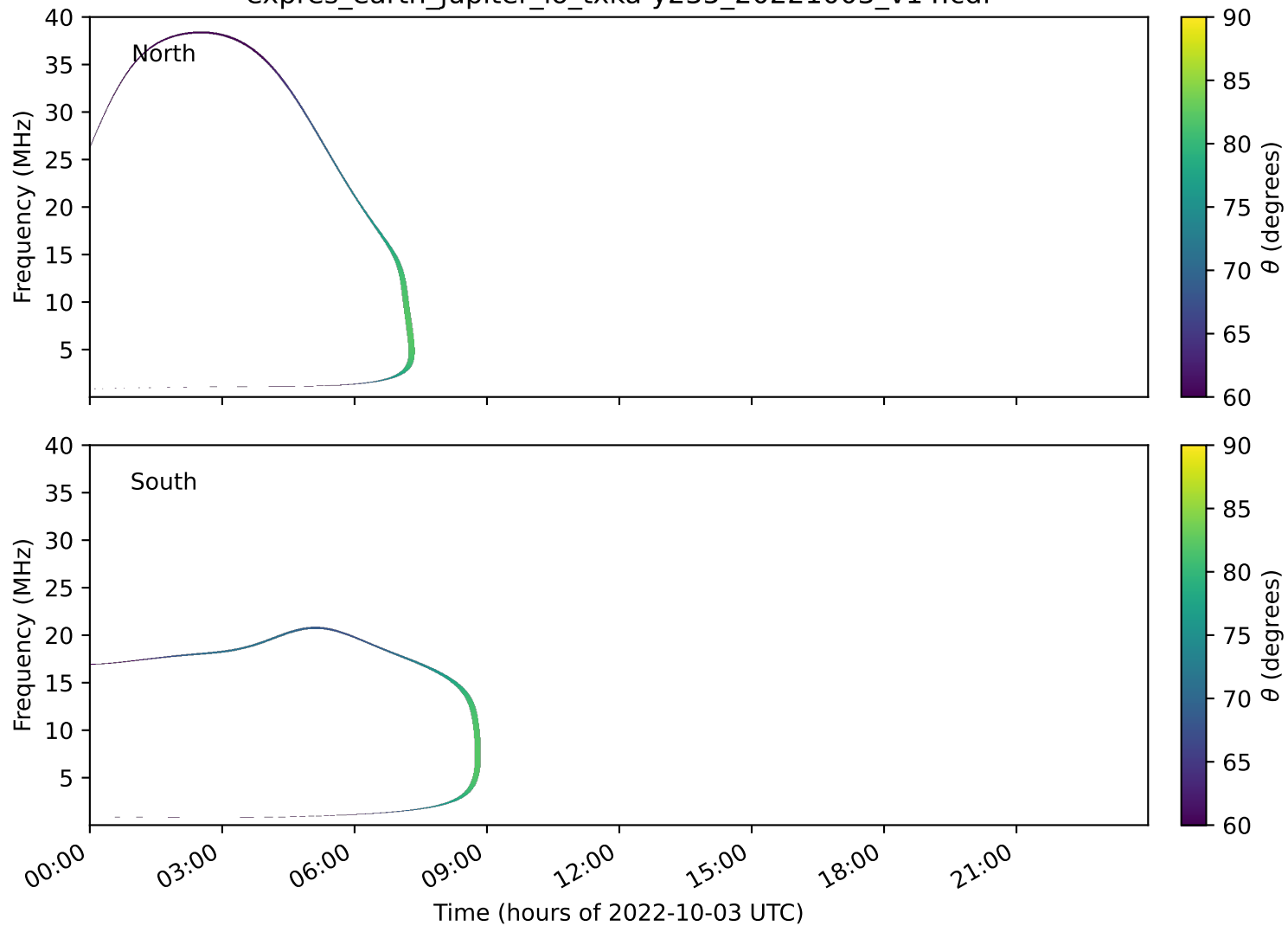
expres_earth_jupiter_io_txka-y235_20221003_v14.cdf
