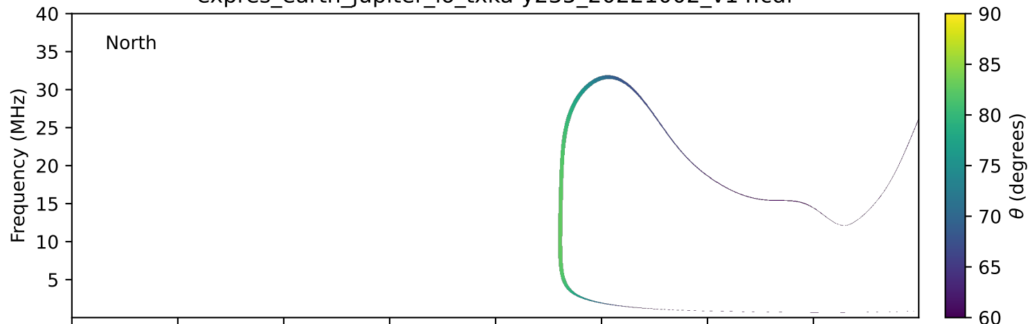
expres_earth_jupiter_io_txka-y235_20221002_v14.cdf
