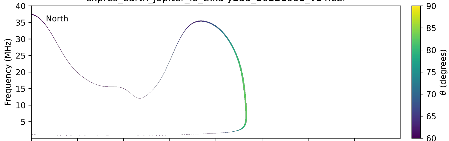
expres_earth_jupiter_io_txka-y235_20221001_v14.cdf
