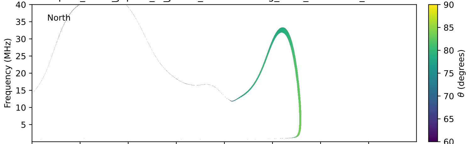
expres_earth_jupiter_io_jrm33_lossc-wid1deg_3kev_20221031_v11.cdf
