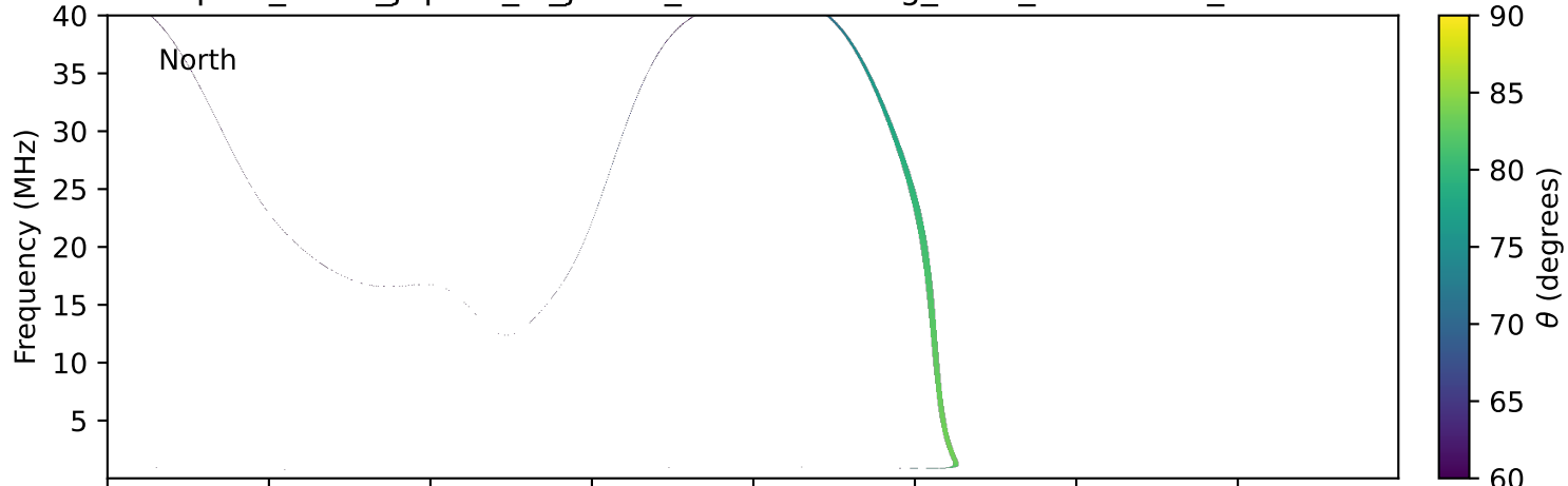
expres_earth_jupiter_io_jrm33_lossc-wid1deg_3kev_20221008_v11.cdf
