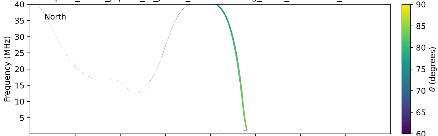
expres_earth_jupiter_io_jrm33_lossc-wid1deg_3kev_20221001_v11.cdf
