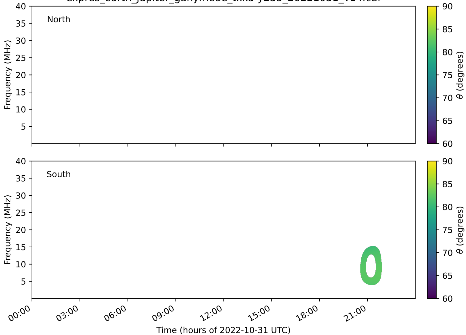
expres_earth_jupiter_ganymede_txka-y235_20221031_v14.cdf
