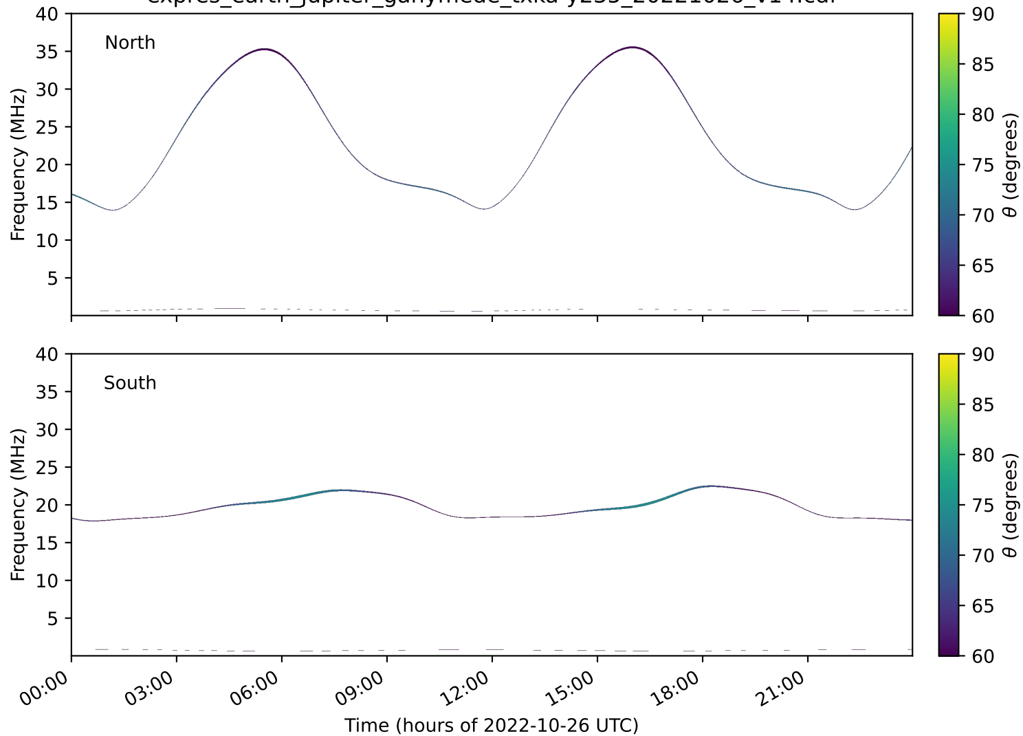
expres_earth_jupiter_ganymede_txka-y235_20221026_v14.cdf
