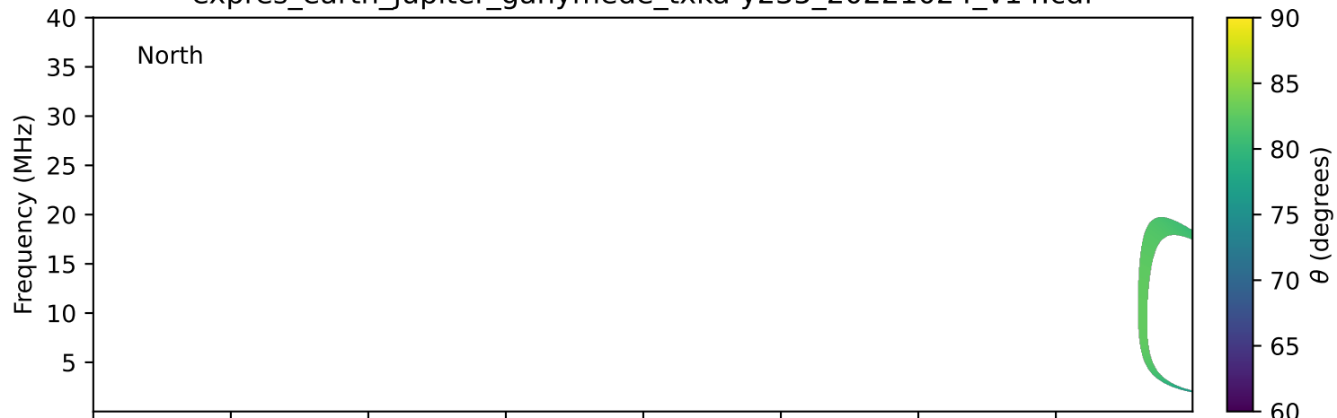
expres_earth_jupiter_ganymede_txka-y235_20221024_v14.cdf
