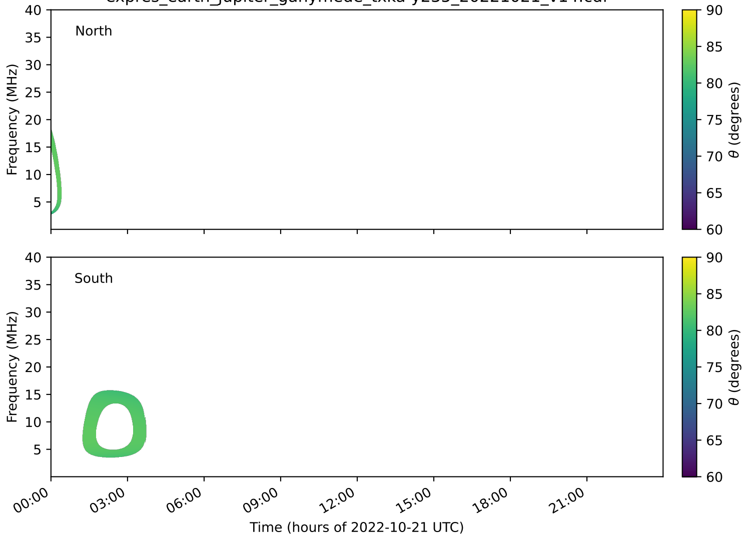
expres_earth_jupiter_ganymede_txka-y235_20221021_v14.cdf
