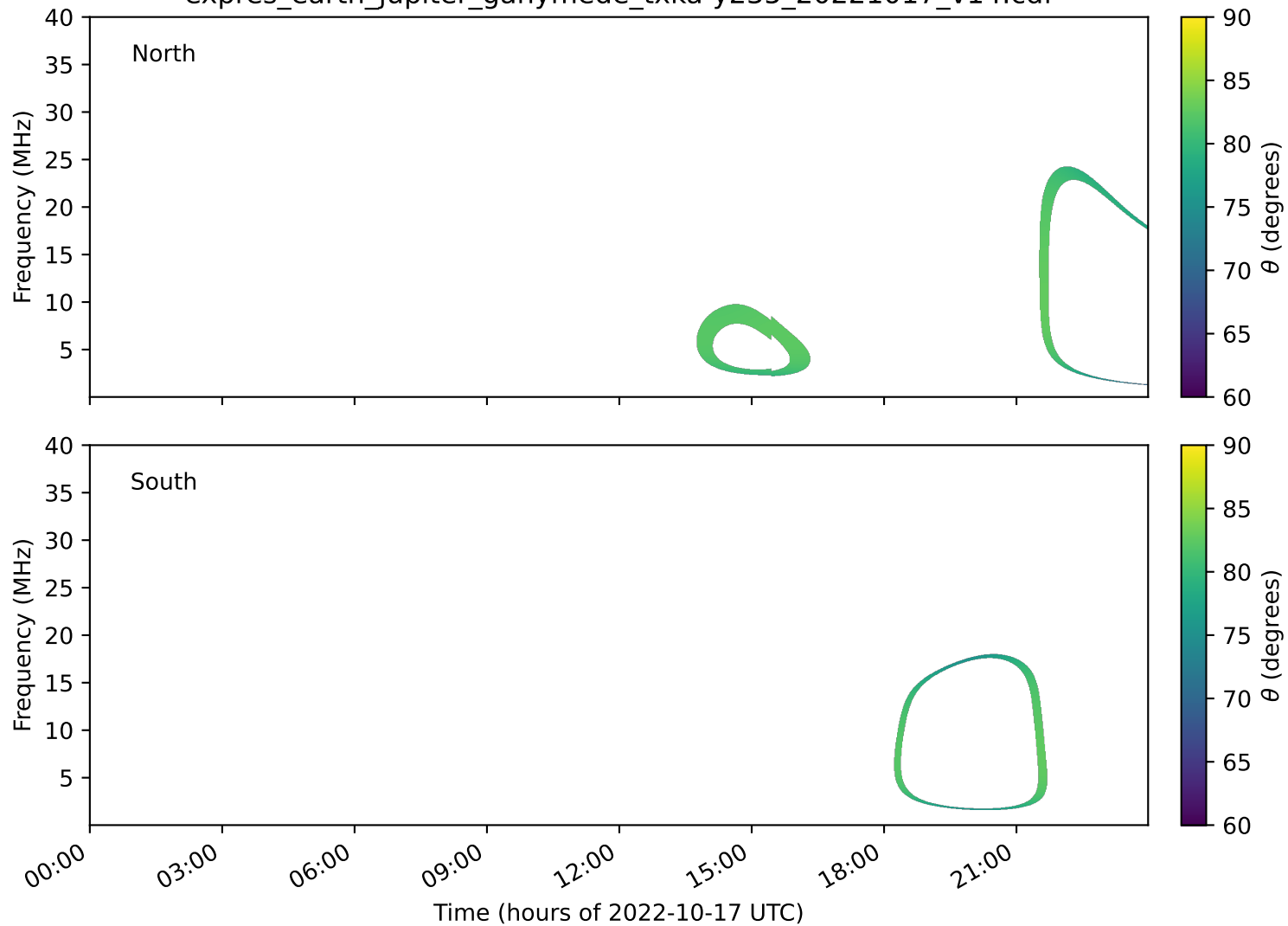
expres_earth_jupiter_ganymede_txka-y235_20221017_v14.cdf
