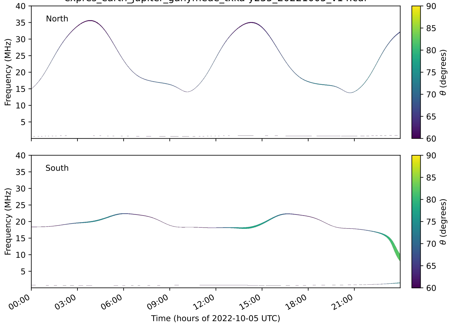
expres_earth_jupiter_ganymede_txka-y235_20221005_v14.cdf
