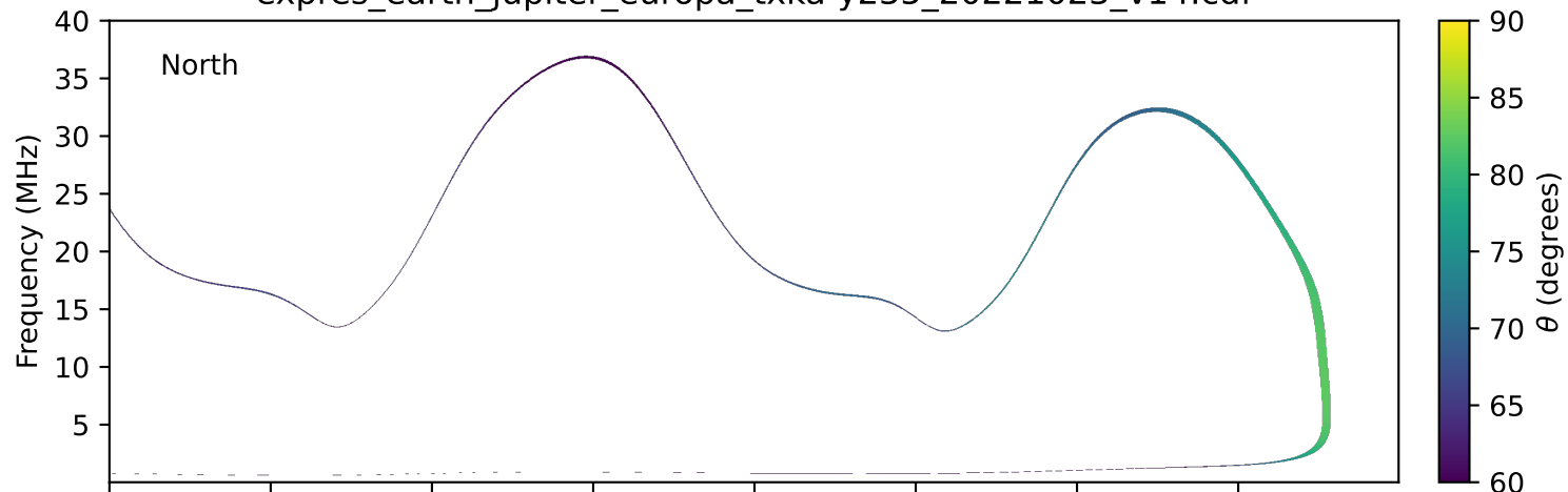
expres_earth_jupiter_europa_txka-y235_20221023_v14.cdf
