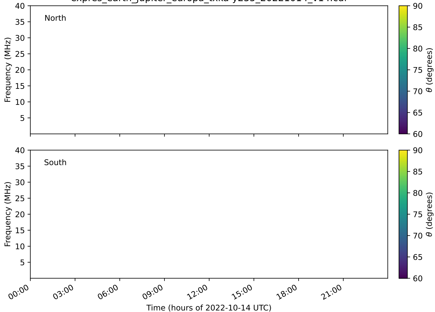
expres_earth_jupiter_europa_txka-y235_20221014_v14.cdf
