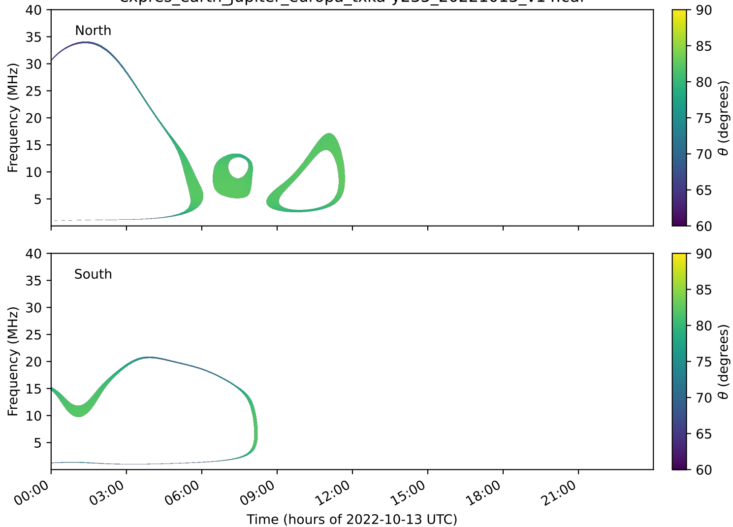
expres_earth_jupiter_europa_txka-y235_20221013_v14.cdf
