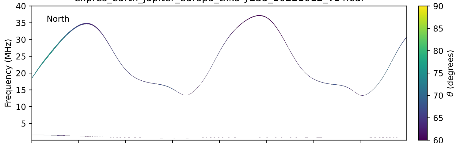
expres_earth_jupiter_europa_txka-y235_20221012_v14.cdf
