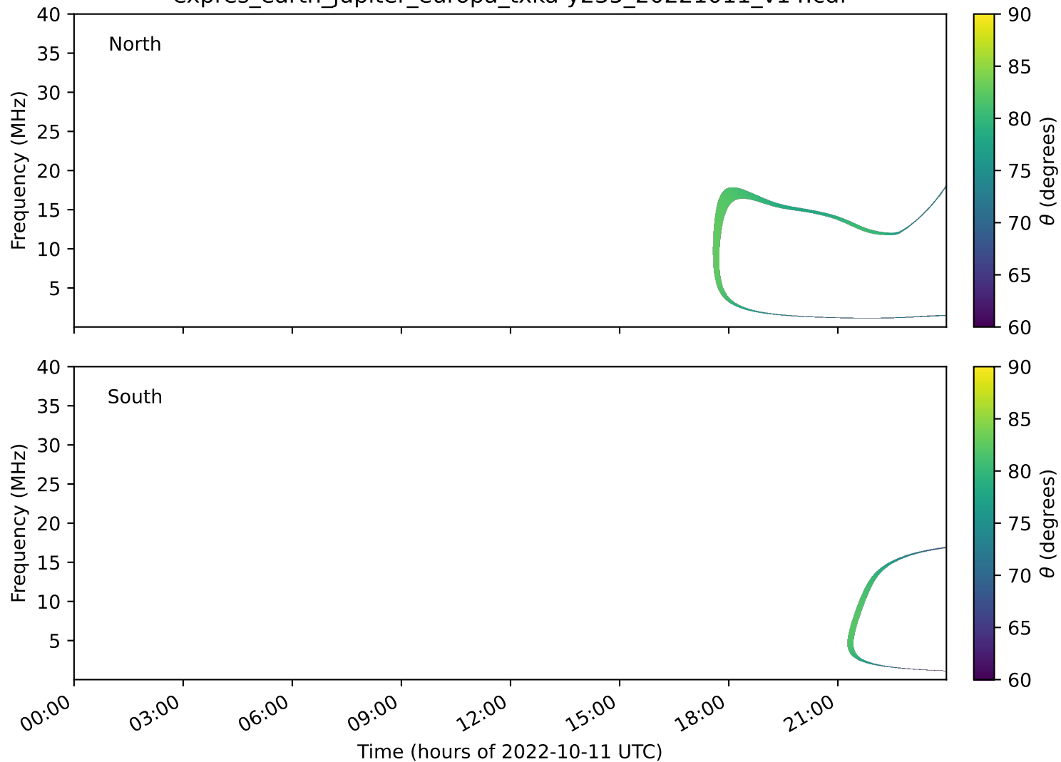
expres_earth_jupiter_europa_txka-y235_20221011_v14.cdf
