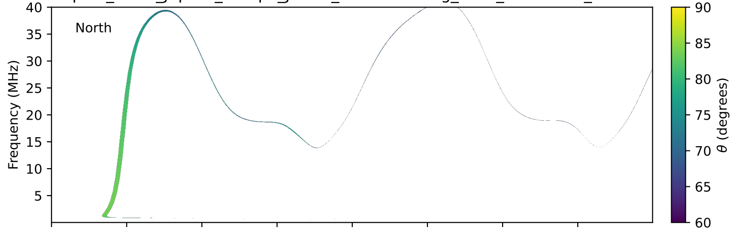
expres_earth_jupiter_europa_jrm33_lossc-wid1deg_3kev_20221026_v11.cdf
